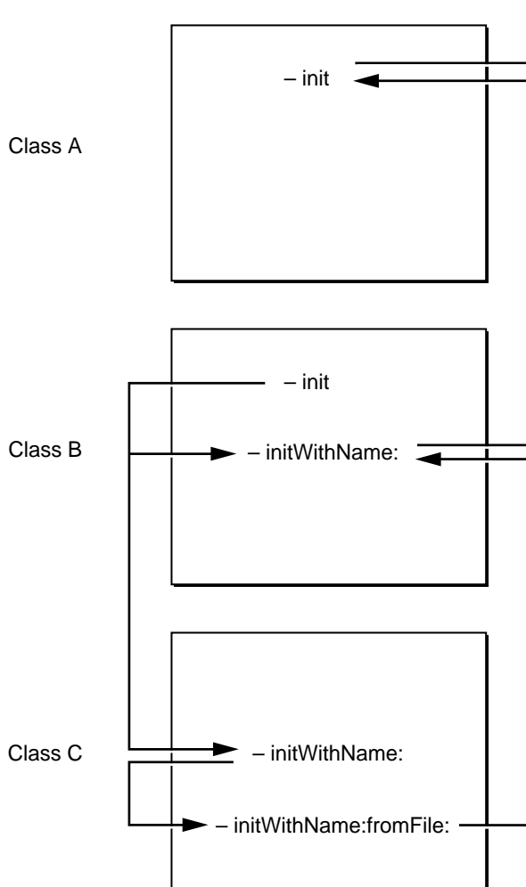
Figure 5-4 Initialization Chain
